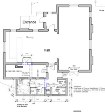
Proposed Plan
